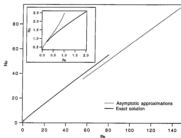
FIGURE 2 The calculated Nusselt number as a function of the Peclet number. The solid curve corresponds to the numerical values of Eq. 5; the dashed curves correspond to asymptotic approximations at low and high \text{Pe} . The inset gives a clear view at low \text{Pe} .
