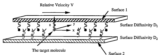
FIGURE 1 Schematic diagram of the system. The target molecule (open circle) is chosen to be on surface 1 and as the origin of the coordinate system. Molecules on surface 1 and surface 2 are assumed to have lateral Brownian motion, which is characterized by diffusion coefficients D_1 and D_2 , respectively. The two surfaces move parallel to each other with a relative velocity V .
