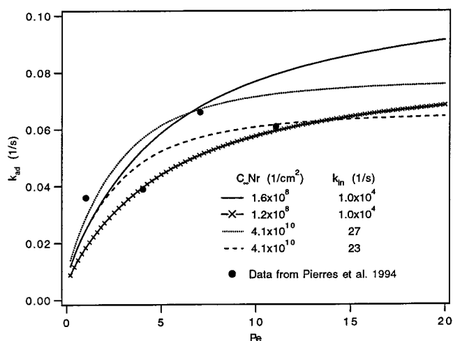
FIGURE 6 Comparison of theoretically calculated overall adhesion rate constants with the experimental values reported by Pierres et al. (1994). The two solid curves (— and -x-) give the range of C_\infty N_r ( 1.2\text{--}1.6 \times 10^8 1/\text{cm}^2 ) for k_{in} = 1.0 \times 10^4 1/\text{s} ; the dashed curve and the dotted curve mark the range of k_{in} (23.0–27.0 1/\text{s} ) for C_\infty N_r = 4.1 \times 10^{10} 1/\text{cm}^2 .
