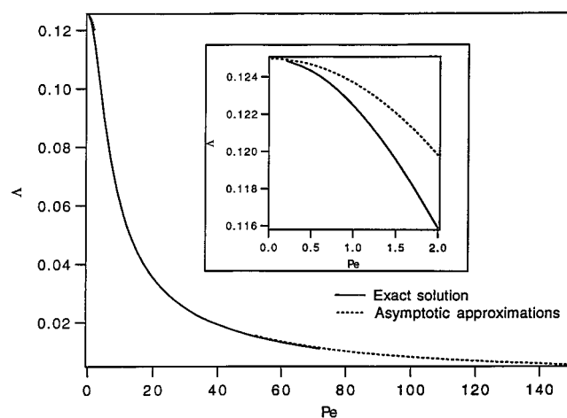
FIGURE 3 The dimensionless duration time, \Lambda , is plotted as a function of the Peclet number. The solid curve corresponds to the numerical values of Eq. 18; the dashed curves correspond to the asymptotes at low and high Pe . The low Pe region is shown in the inset.
